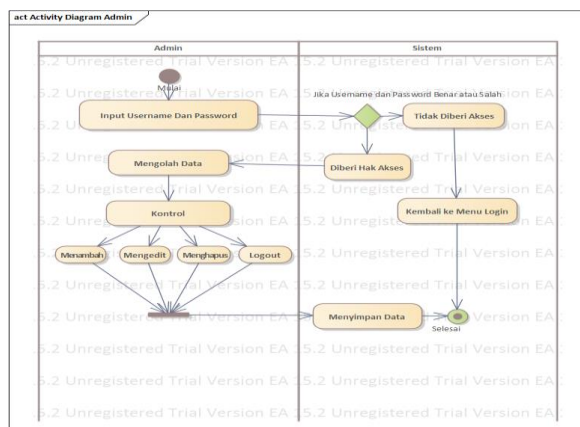
Gambar 3b. Activity Diagram Admin
