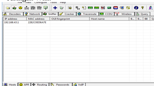
Gambar 3 Start Sniffer
