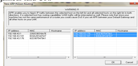
Gambar 7 Block IP
