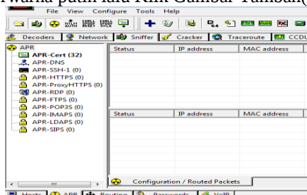
Gambar 6 Start APR
