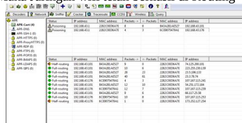
Gambar 9 Hasil Routing
